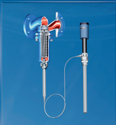
Thermal-closing valve
